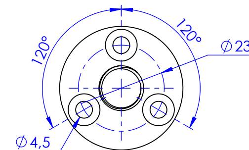
Platine de fixation. Fixing plate.
